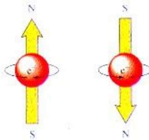
Spinning electron
