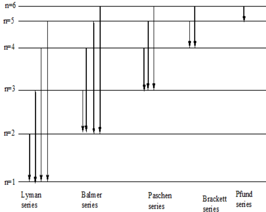
Various series in hydrogen spectrum.
