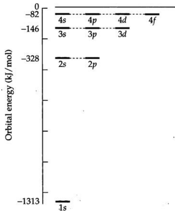
(a) Hydrogen
