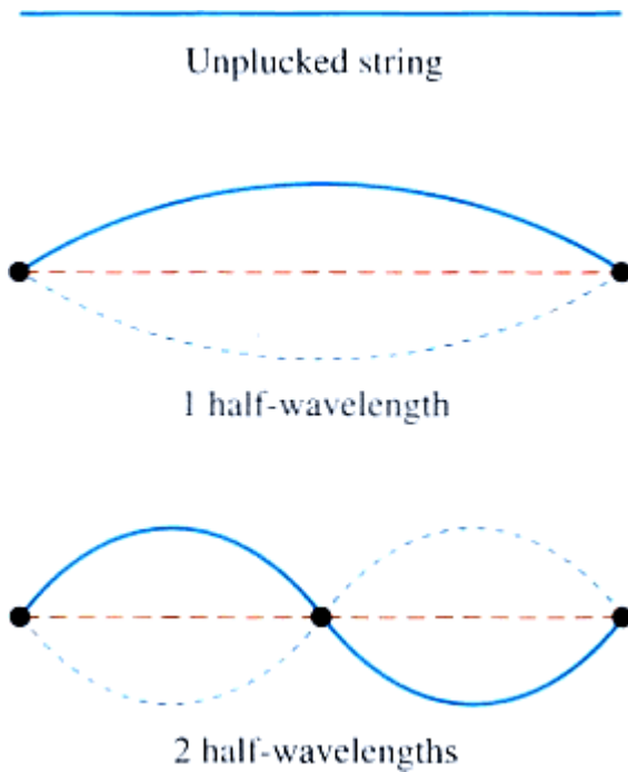
Standing wave
